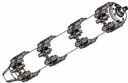
Submersible motor fitted with anode strings
